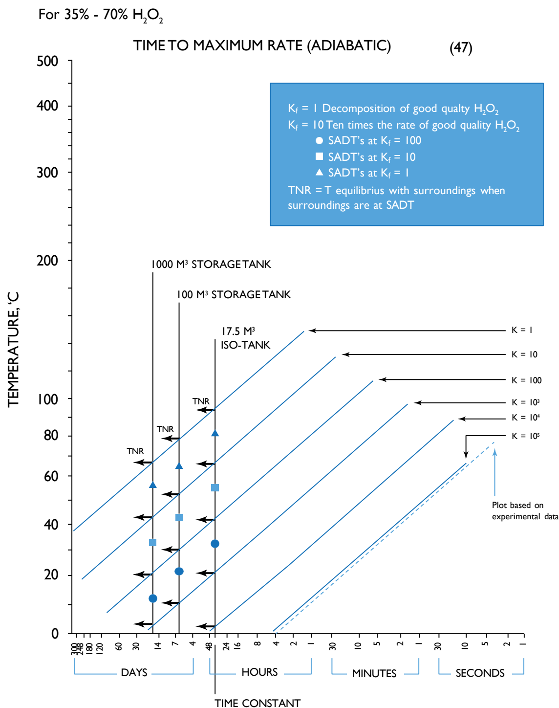
FIGURE 2 - T.N.R. 'S AND S.A.D.T. 'S FOR TYPICAL 100 m 3 AND 1000 m 3 TANKS AND 17.5 m 3 I.S.O. TRANSPORT TANK
